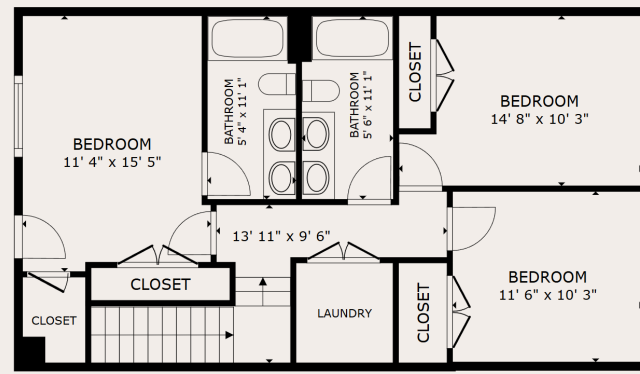
LOT 4 - FLOOR 2
