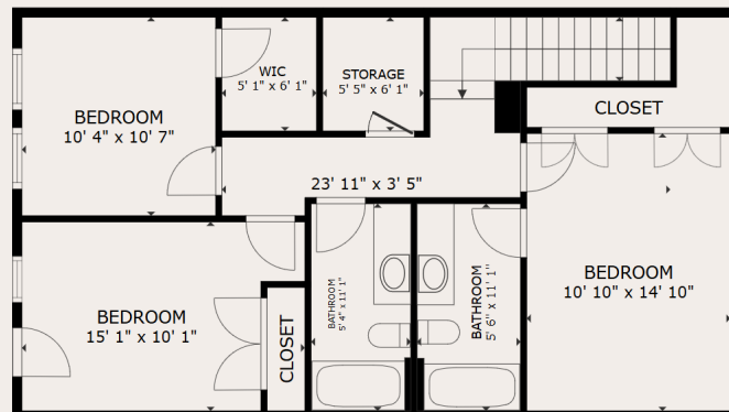
LOT 5 - FLOOR 2
